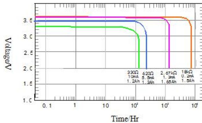
Different load discharge characteristics at normal temperature 常温下不同负载放电特性
