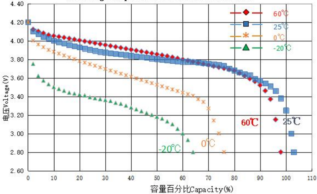
Discharge temperature characteristics curve
