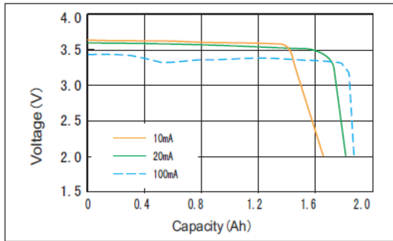
Discharge characteristics at 150°C
