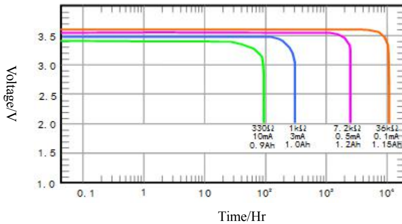
Different load discharge characteristics at normal temperature 常温下不同负载放电特性
